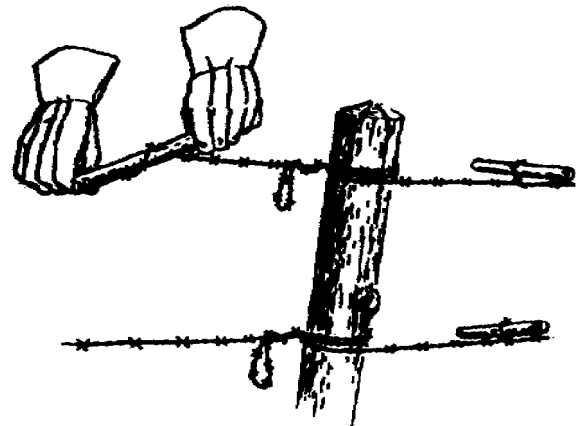
Figure 4-18. Tightening wire by racking.
